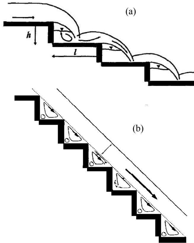
Fig. 3: Different regimes over stepped spillways; a) Jet or nappe flow, b) skimming flow.
