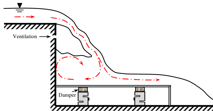
Fig. 5: Reducing the impact force of the falling jet by using dampers.
