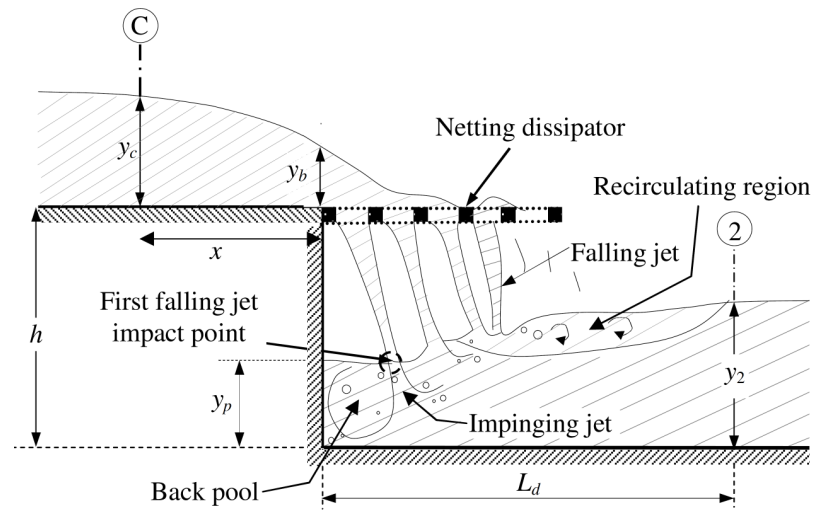
Fig. 4: Inserting a net at the brink section to increase the energy loss.
