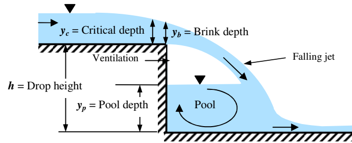
Fig. 1: Definition sketch of flow over a drop.
